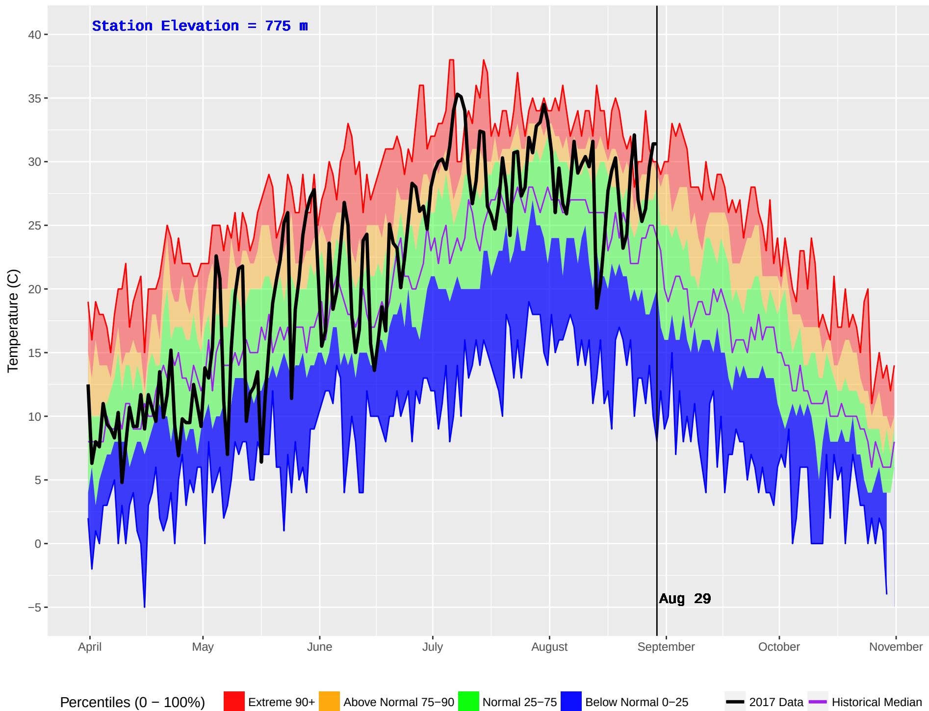
ELKO (412) : Historical (1970–2016) and Current (2017) Noon Temperature
